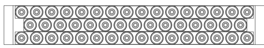
HVGP60(HSCN20)SUCKER DIAMETER 20MM 3-row arrangement types of: PX03
